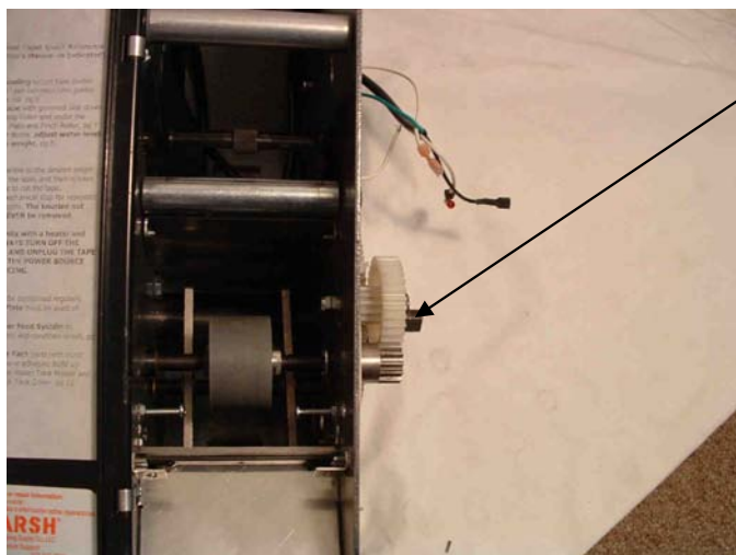
Fig 20 Idler Gear
