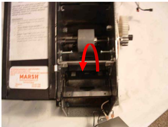
Fig 19 Movable Cutter Assembly
