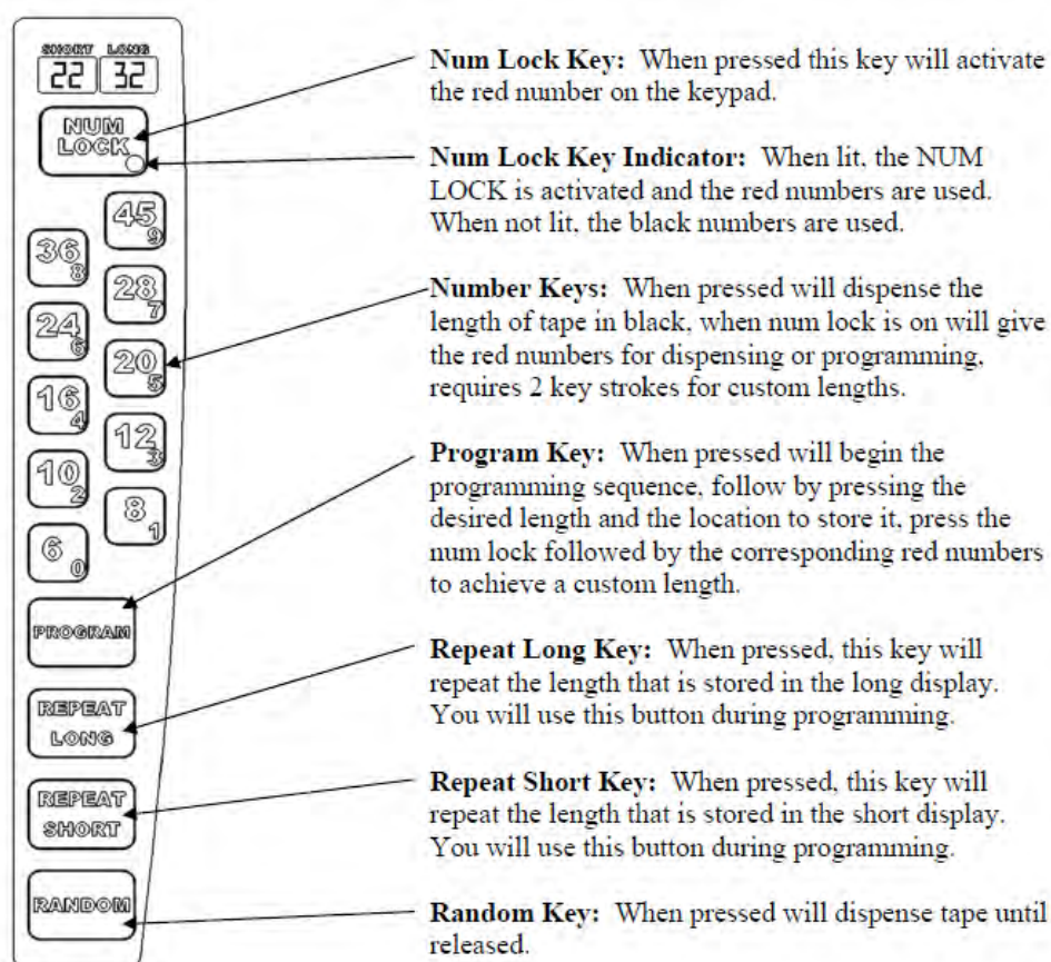
Figure 7 – Premium Short Keypad
