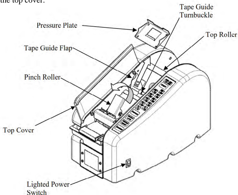
Figure 2 – Loading Tape
