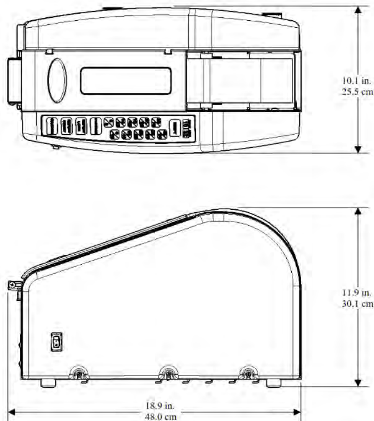
Figure 1 – Tape Machine Dimensions
