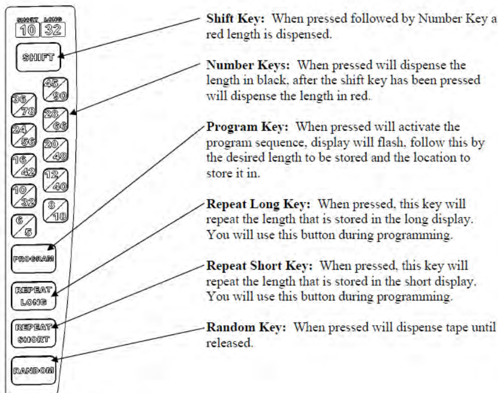
Figure 6 – Standard Keypad
